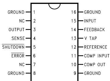
Figure 6. LP2953 16-Pin
