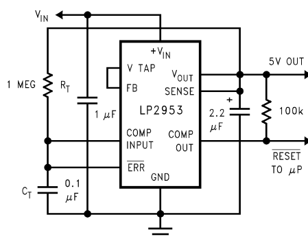
Figure 17. 5V Regulator with Timed Power-On Reset
