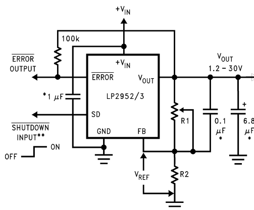
Figure 10. Adjustable Regulator
