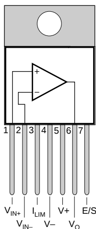
7-Lead Straight-Formed TO-220 (T-1)
