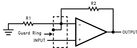
Figure 8. Non-Inverting Amplifier Typical Connections of Guard Rings
