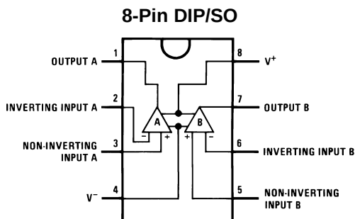
Figure 1. Top View
