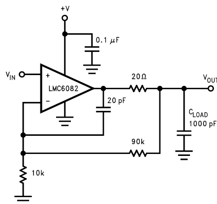
Figure 4. LMC6082 Noninverting Gain of 10 Amplifier, Compensated to Handle Capacitive Loads
