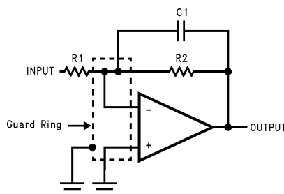
Figure 7. Inverting Amplifier Typical Connections of Guard Rings
