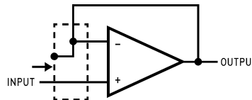
Figure 9. Follower Typical Connections of Guard Rings
