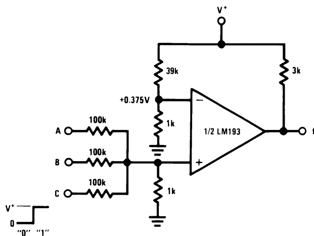
Figure 19. AND Gate
