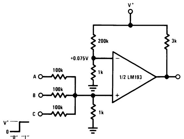
Figure 20. OR Gate
