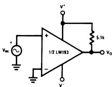
Figure 29. Zero Crossing Detector
