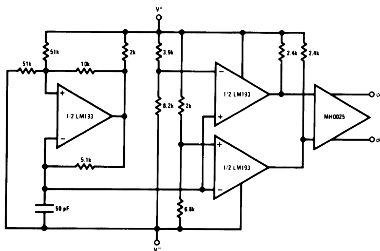
Figure 32. MOS Clock Driver
