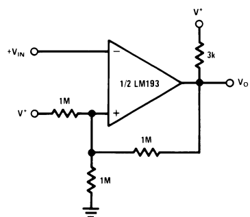
Figure 17. Inverting Comparator with Hysteresis
