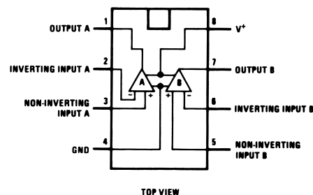
Figure 5. Dual-In-Line/SOIC Package
