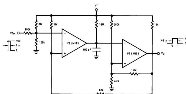
Figure 28. One-Shot Multivibrator with Input Lock Out
