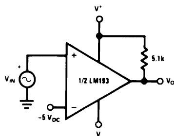
Figure 30. Comparator With a Negative Reference
