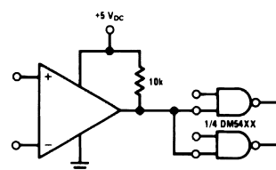
Figure 10. Driving TTL
