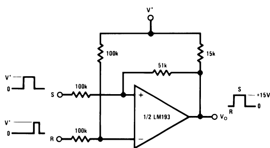
Figure 27. Bi-Stable Multivibrator
