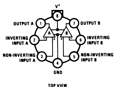
Figure 4. Metal Can Package
