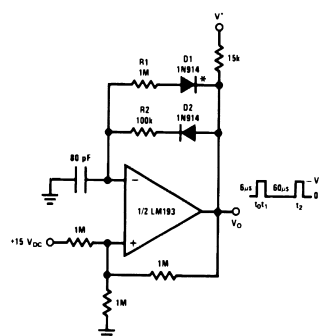
Figure 11. Squarewave Oscillator
