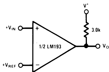
Figure 15. Basic Comparator
