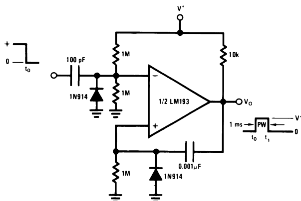
Figure 26. One-Shot Multivibrator
